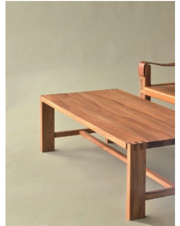
Cross bar coffee table T06 W1130 D330 H350mm
